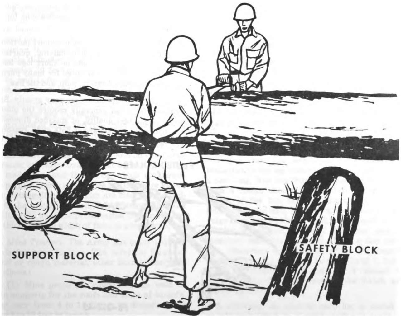
Figure 6-6. Method of propping and bucking a log.
